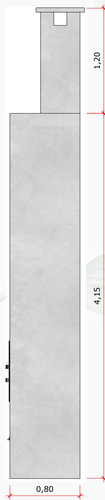
VISTA LATERAL CHURRASQUEIRA ESCALA 1.:25
