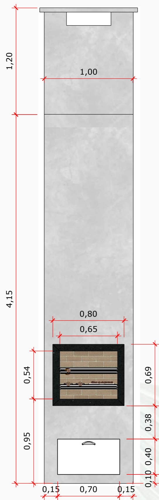
VISTA FRONTAL CHURRASQUEIRA ESCALA 1.:25
