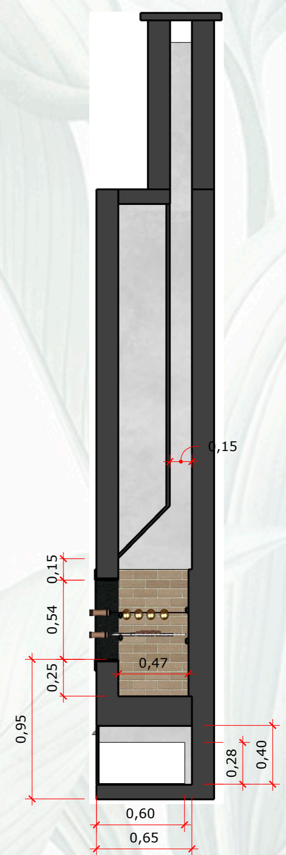
CORTE CHURRASQUEIRA ESCALA 1.:25
